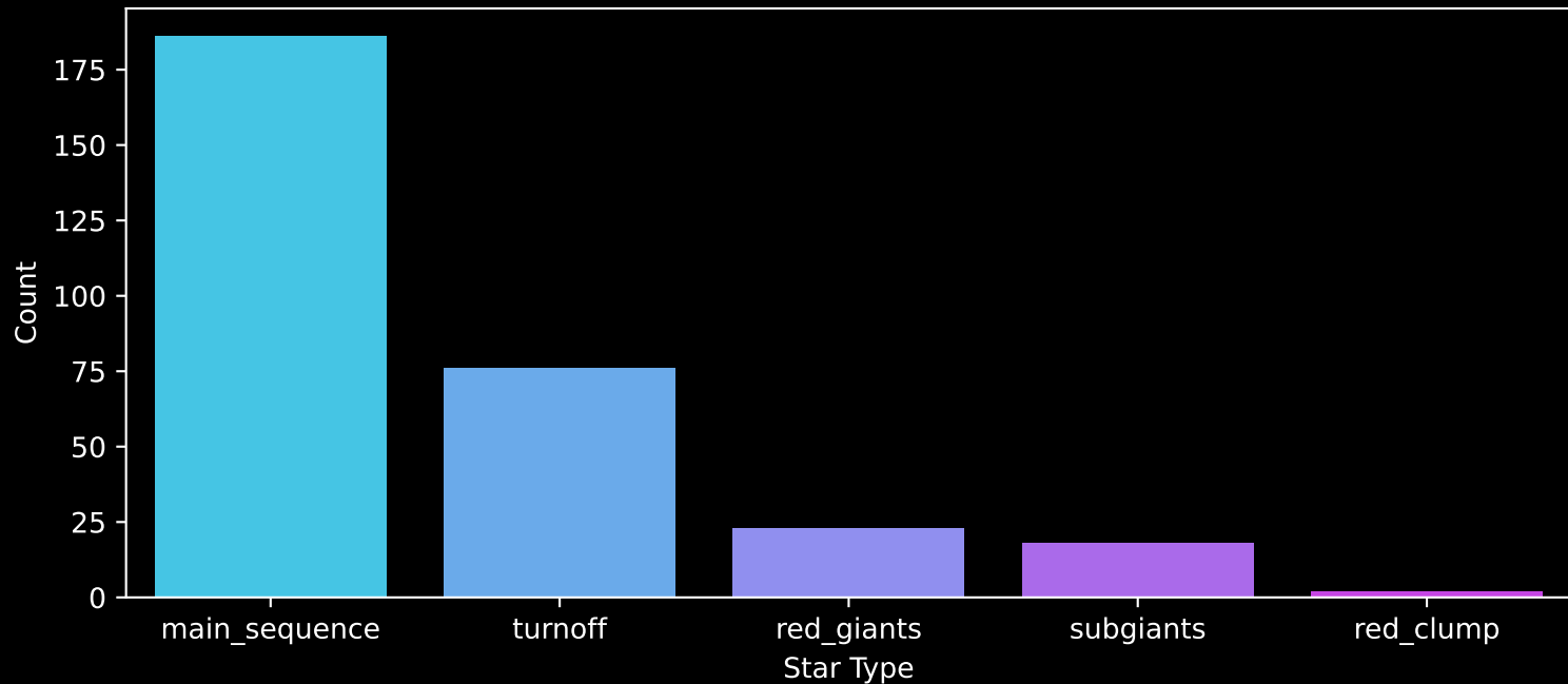
GALAH DR4 Field: [6966] Count plot of Star Type
