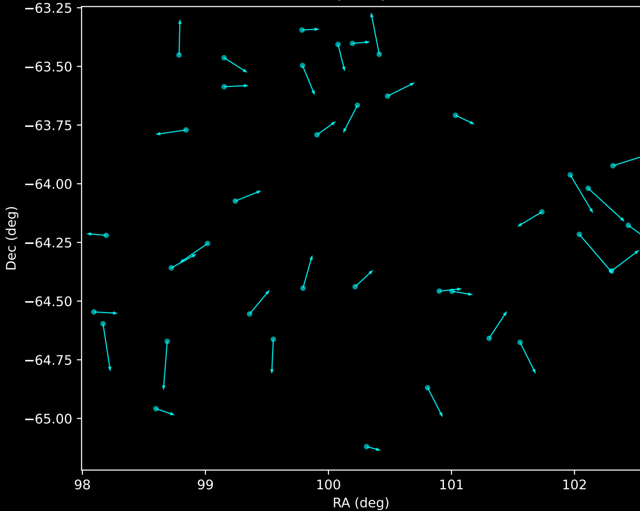
GALAH DR4 Noise Stream Proper Motion Vectors (n=38)
