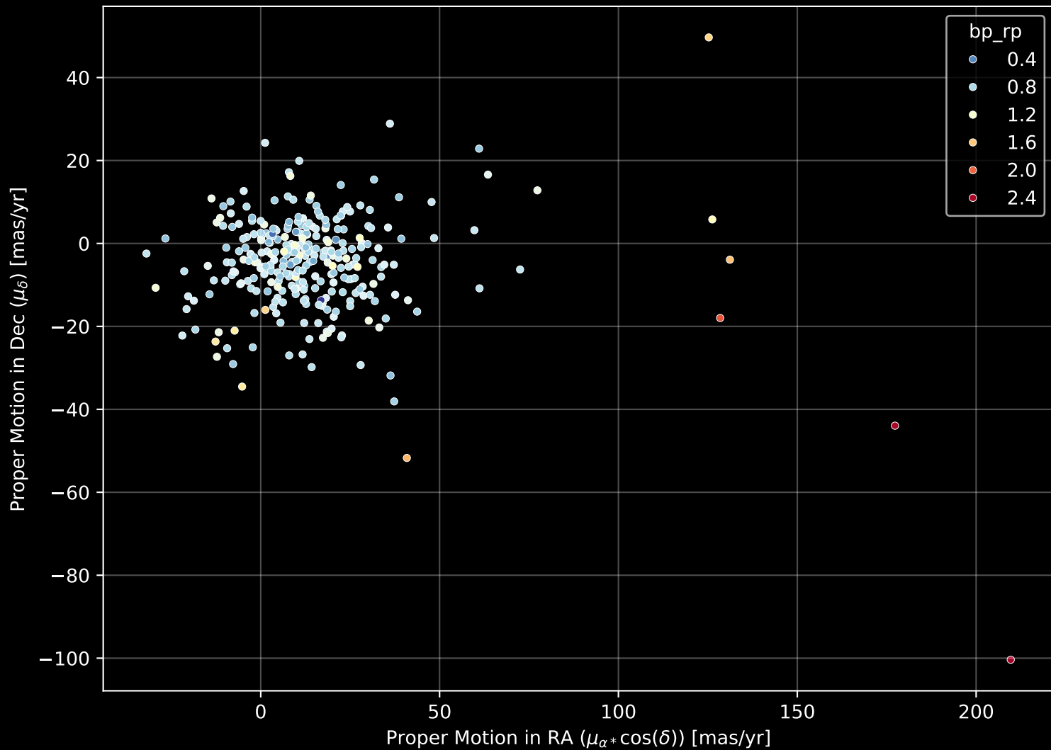
GALAH DR4 Field: [6966] Proper Motion Diagram (n= 305)
