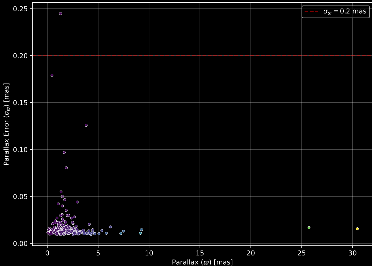
GALAH DR4 Field: [6966] Parallax Quality (n= 305)
