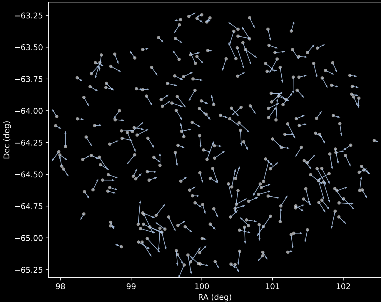
GALAH DR4 Cluster 1 Proper Motion Vectors (n=260)
