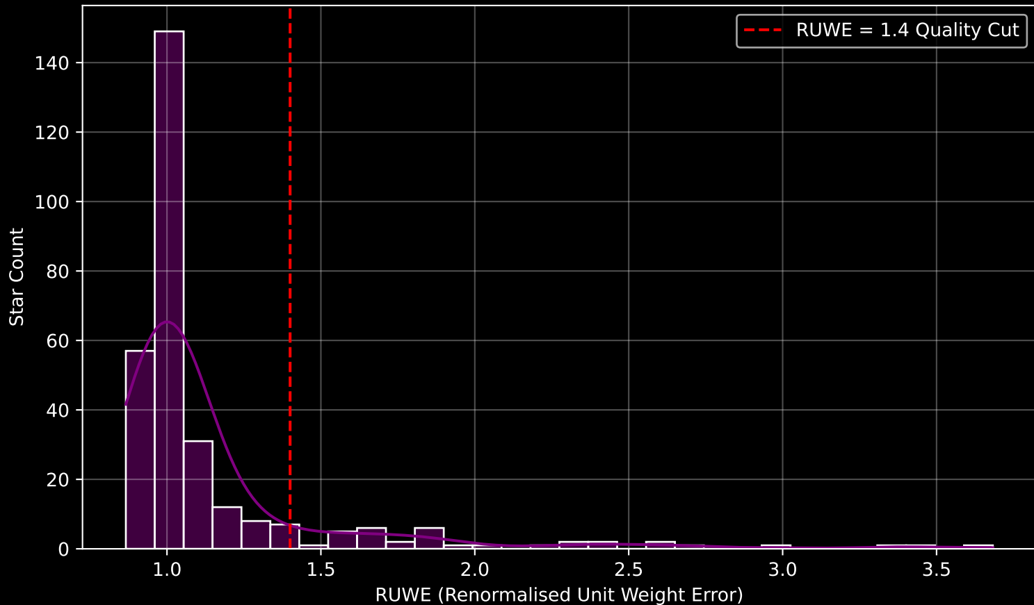
GALAH DR4 Field [6966] RUWE Distribution (n= 298)
