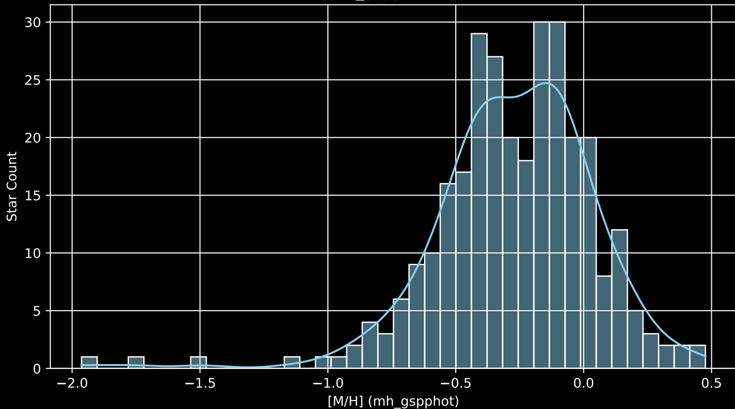
GALAH DR4 Field: [6966] [M/H] (mh_gspphot) (n= 301)
